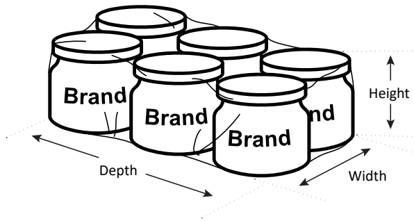
Figure 5-4 Dimensions of non-consumer trade items (shrink pack)
