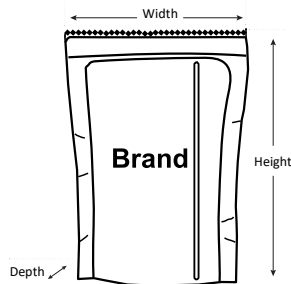
Figure 4-13 Stand up pouches
