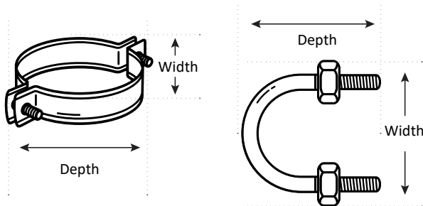
Figure 4-90 Loose pipe hanger measurements.
