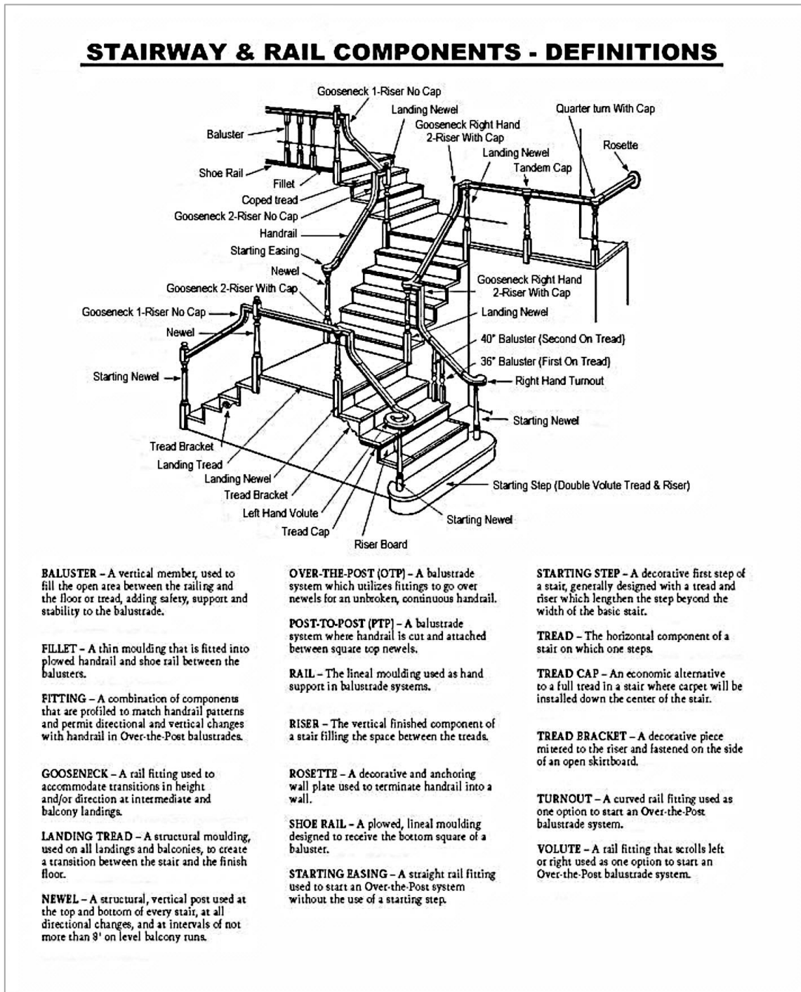
Figure A-1 Illustration reprinted with permission of Crown Heritage Stair Company
