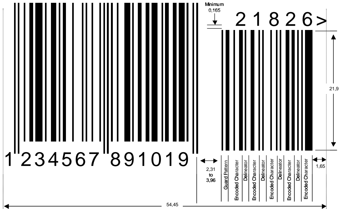
Figure 5.2.4.6 - 7 EAN-13 Bar Code Symbol with Five-Digit Add-On Symbol
