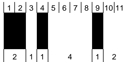
Figure 5.4.3.1 - 1 GS1-128 Bar Code Symbol Start Character A
