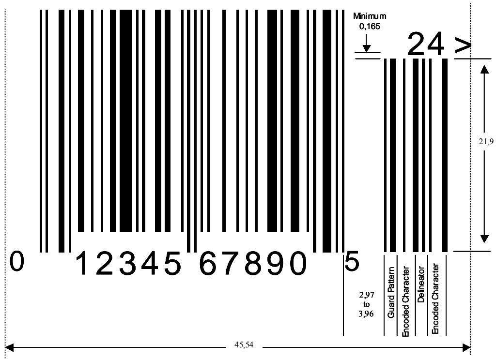
Figure 5.2.4.6 - 6 UPC-A Bar Code Symbol with Two-Digit Add-On Symbol
