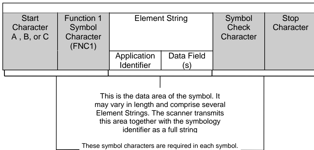
Figure A1 - 1 Example GS1-128 Bar Code Symbol Structure
