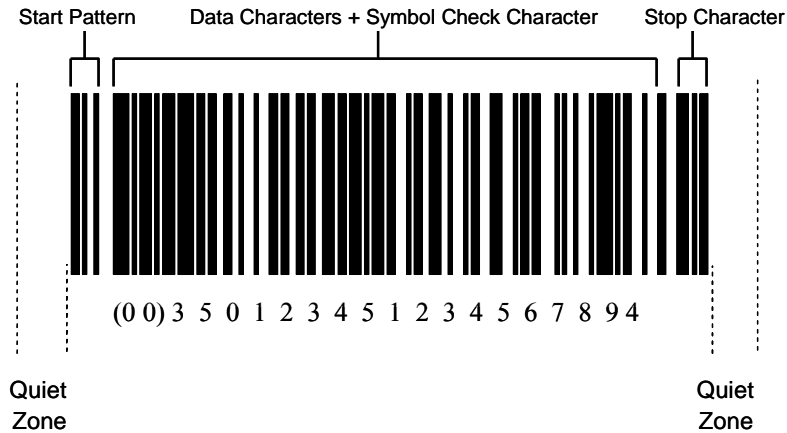
Figure 5.4.2 - 1 General Format of a GS1-128 Bar Code Symbol
