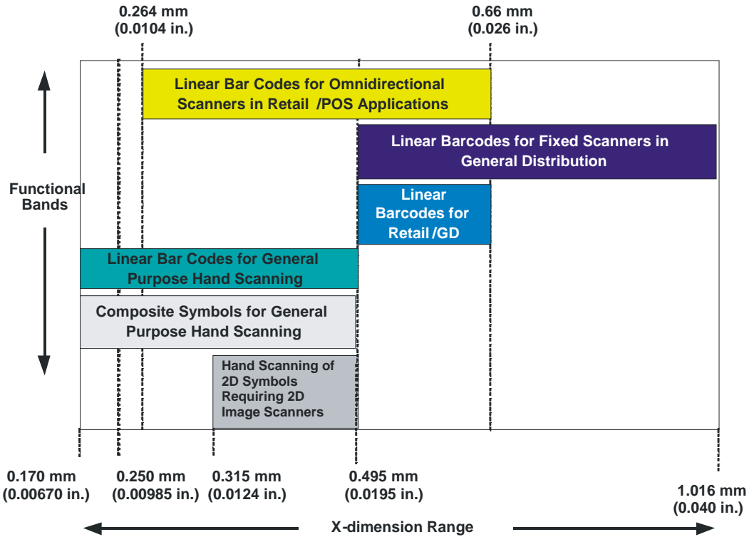
Figure 5.5.2.6.1 - 1 GS1 Scanner Functional Operative Bands
