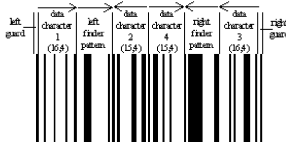
Figure 5.6.1.2 - 1 First Group of GS1 DataBar Symbols Structure
