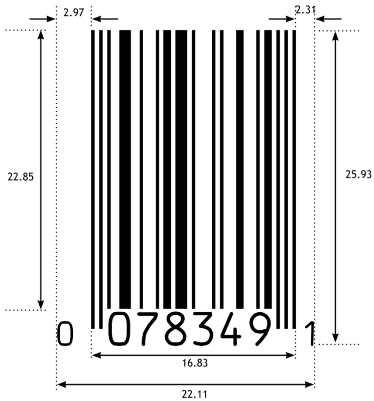
Figure 5.2.4.6-4. UPC-E barcode
