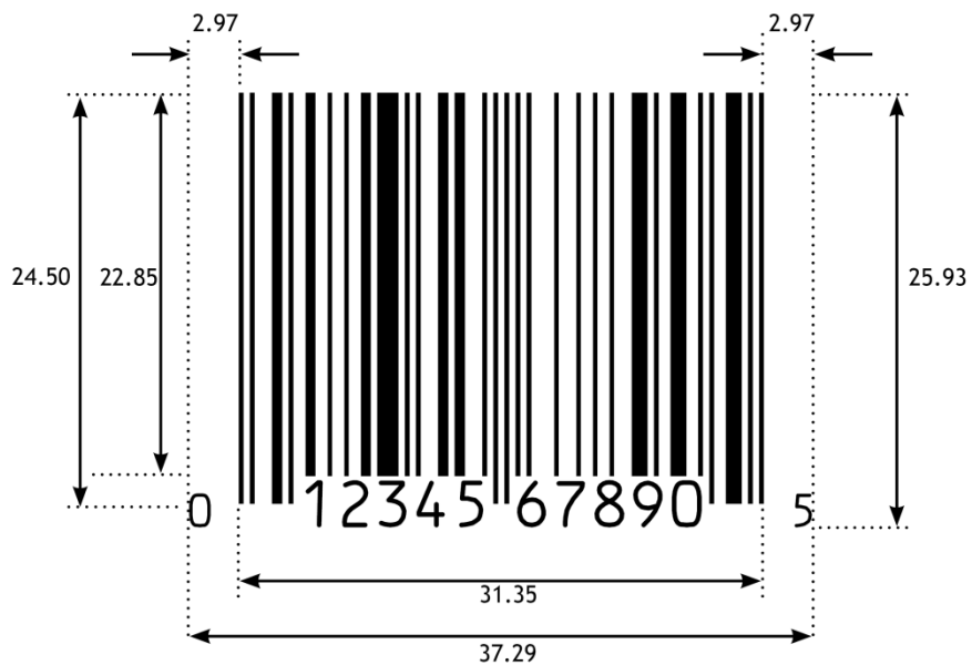
Figure 5.2.4.6-2. UPC-A barcode
