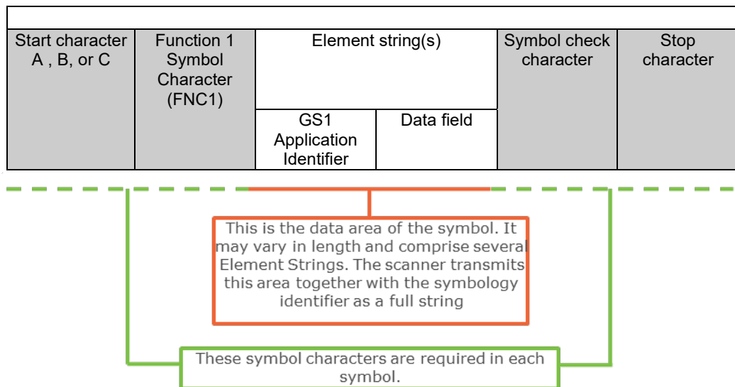
Figure 5.10.1-1. Example GS1-128 barcode structure
