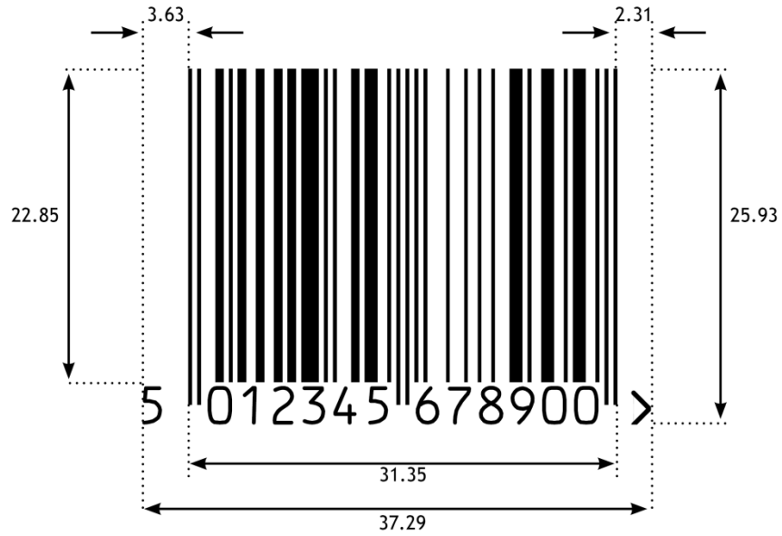
Figure 5.2.4.6-1. EAN-13 barcode
