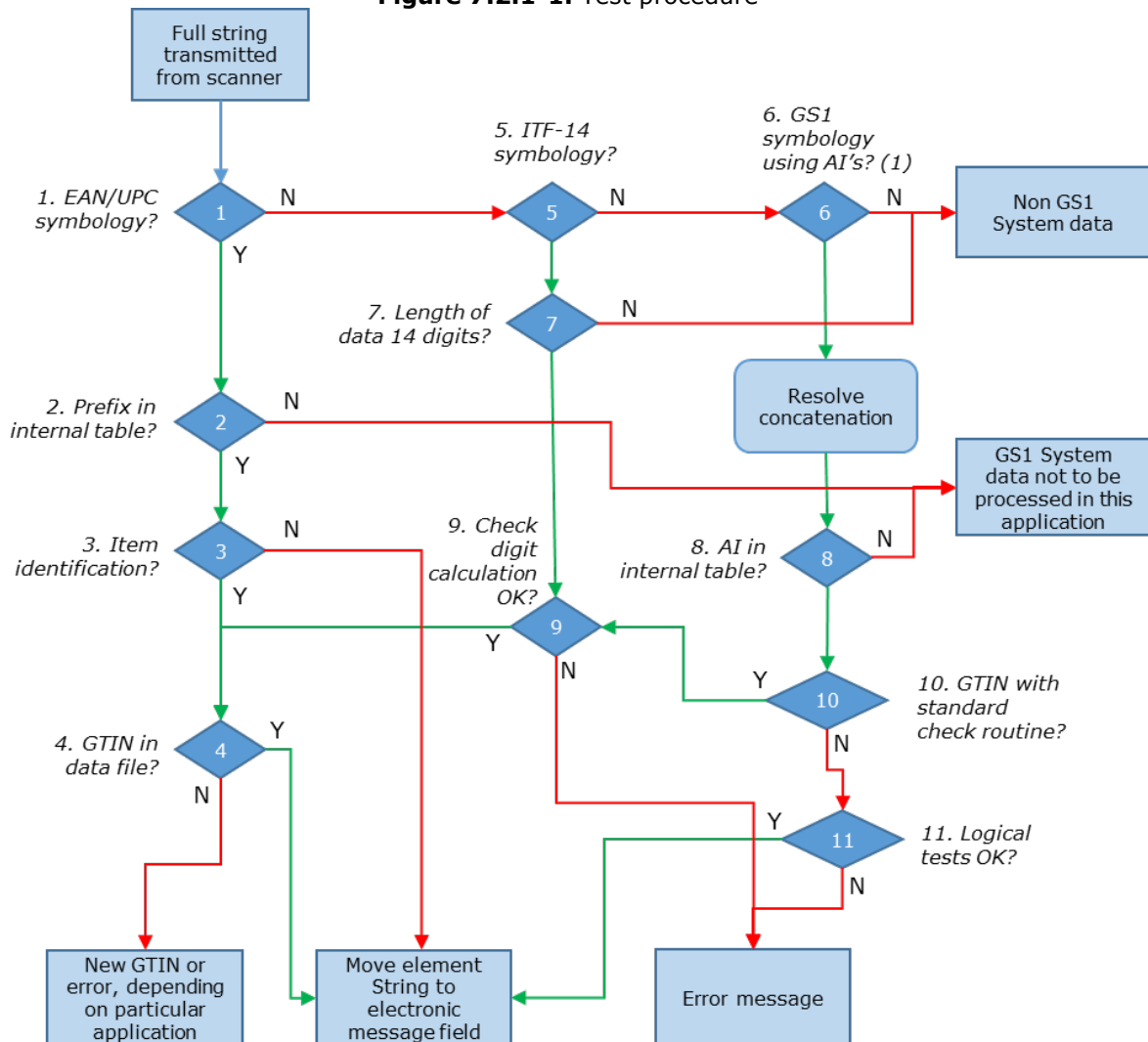
Figure 7.2.1-1. Test procedure
