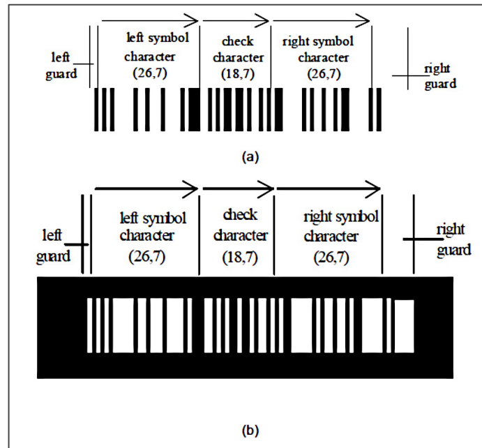
Figure 5.6.2.2-2. GS1 DataBar Limited barcode structure
