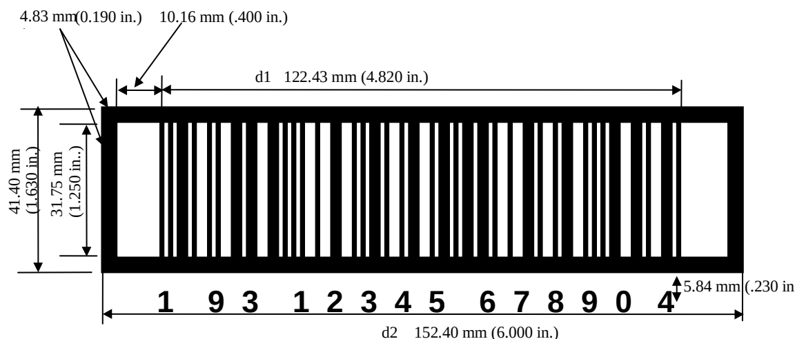
Figure 5.3.1.10-1. ITF-14 Symbol: Main Dimensions at X-dimension 1.016 mm (0.0400 in.)
