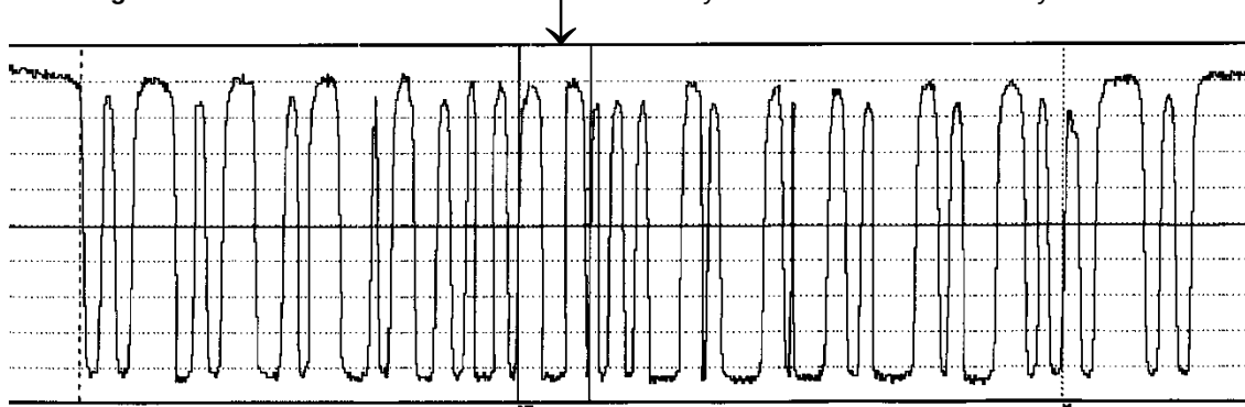
Figure 5.5.3.3.12-4. Scan Reflectance Profile of Symbol with Low Decodability Character
