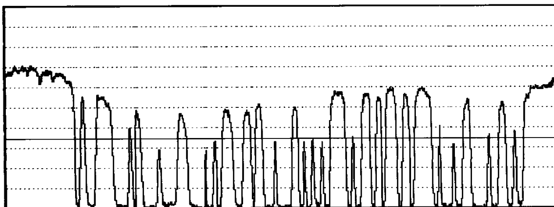
Figure 5.5.3.3.12-2. Scan Reflectance Profile with Narrow Space Profiles
