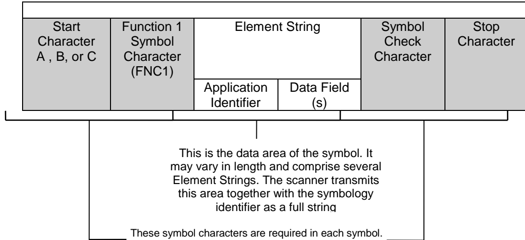
Figure A1 – 1. Example GS1-128 Bar Code Structure
