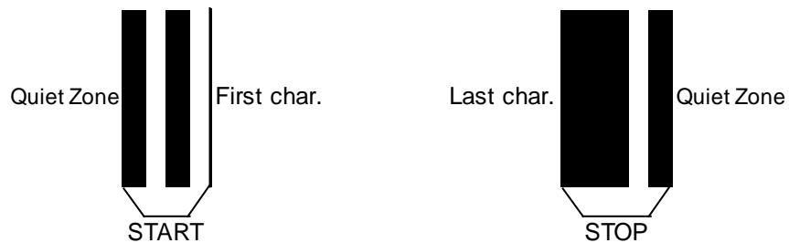
Figure 5.3.1.2.2 – 1. Start and Stop Patterns
