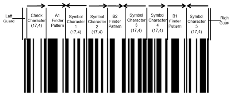
Figure 5.6.1.4 - 1 GS1 DataBar Expanded Structure
