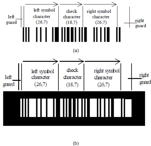
Figure 5.6.1.3 - 2 GS1 DataBar Limited Bar Code Structure
