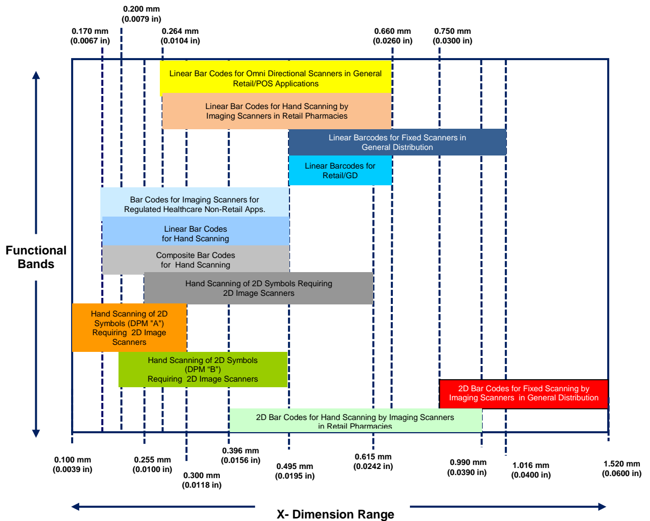
Figure 5.5.2.6.1 - 1 GS1 Scanner Functional Operative Bands
