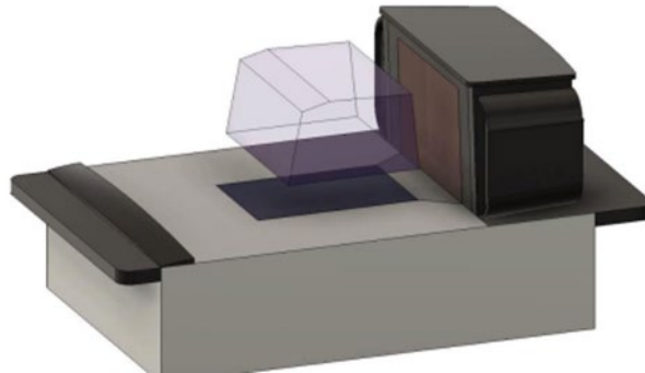
Figure 5-1 Bi-optic scanner barcode scan path example
