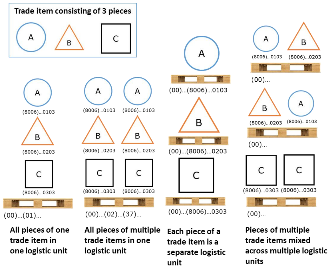
Figure 4-2 Identification of pieces of a trade item
