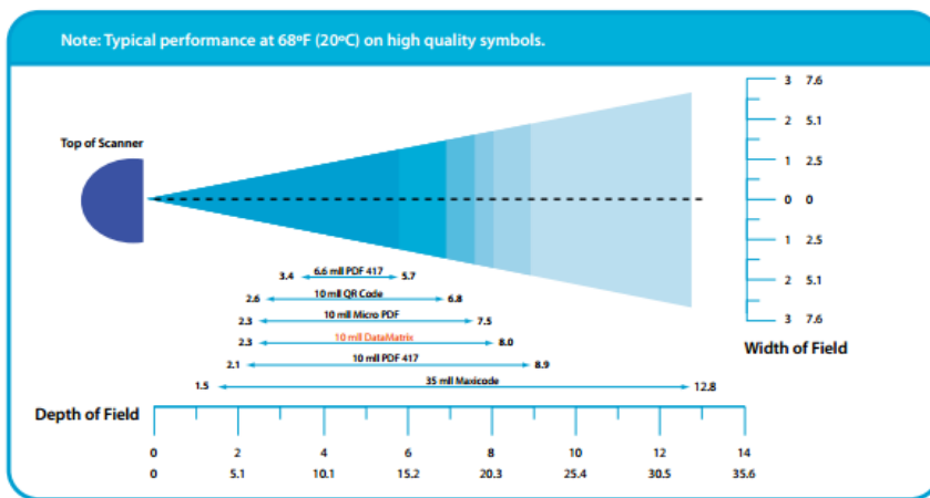
Figure 3-2 Typical reading distance and the depth of a scanner
