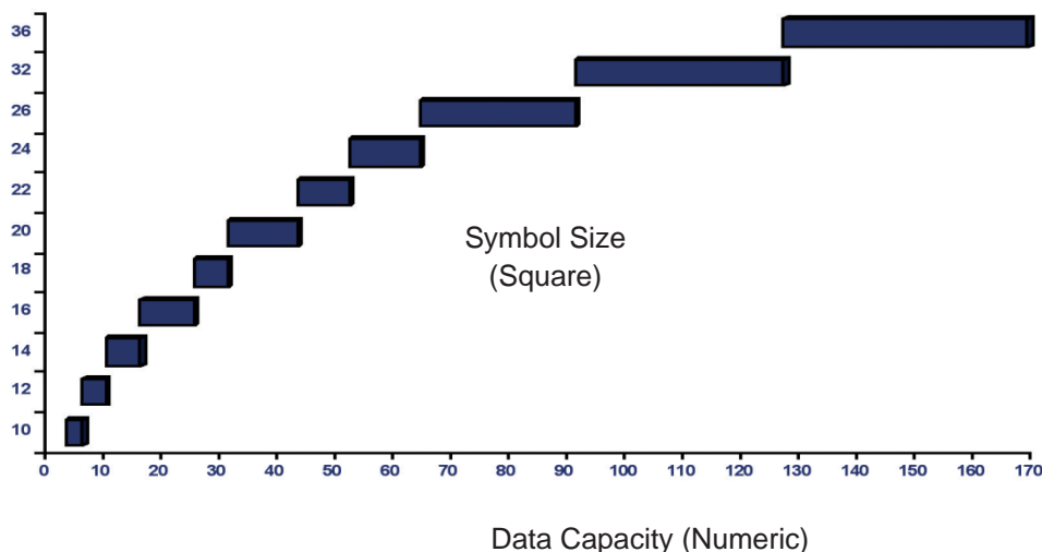
Figure 1.2.2-1 Symbol Size vs. Numeric Capacity
