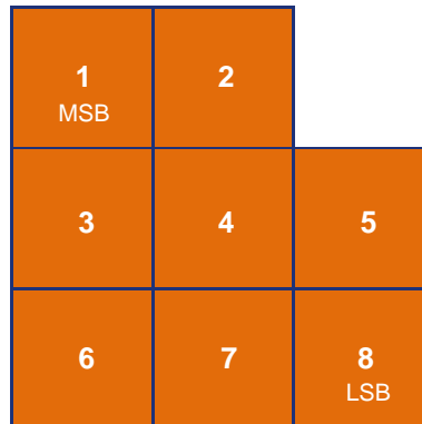
Figure 6 Representation of a codeword in a symbol character for ECC 200
