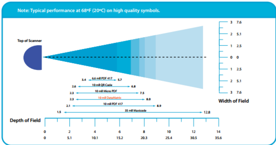
Figure 3.2.2.3-1 Typical Reading distance and the depth of a scanner
